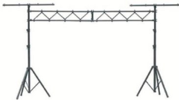
SoundKing DA010 - Aluminium FLAT Truss Lighting Stand System with 2 x T Bars (38*1220mm), 1620-3250mm height adjustment, 1500mm/3000mm flat truss middle (38mm), 100kg load capacity (Formerly LTS30T)
